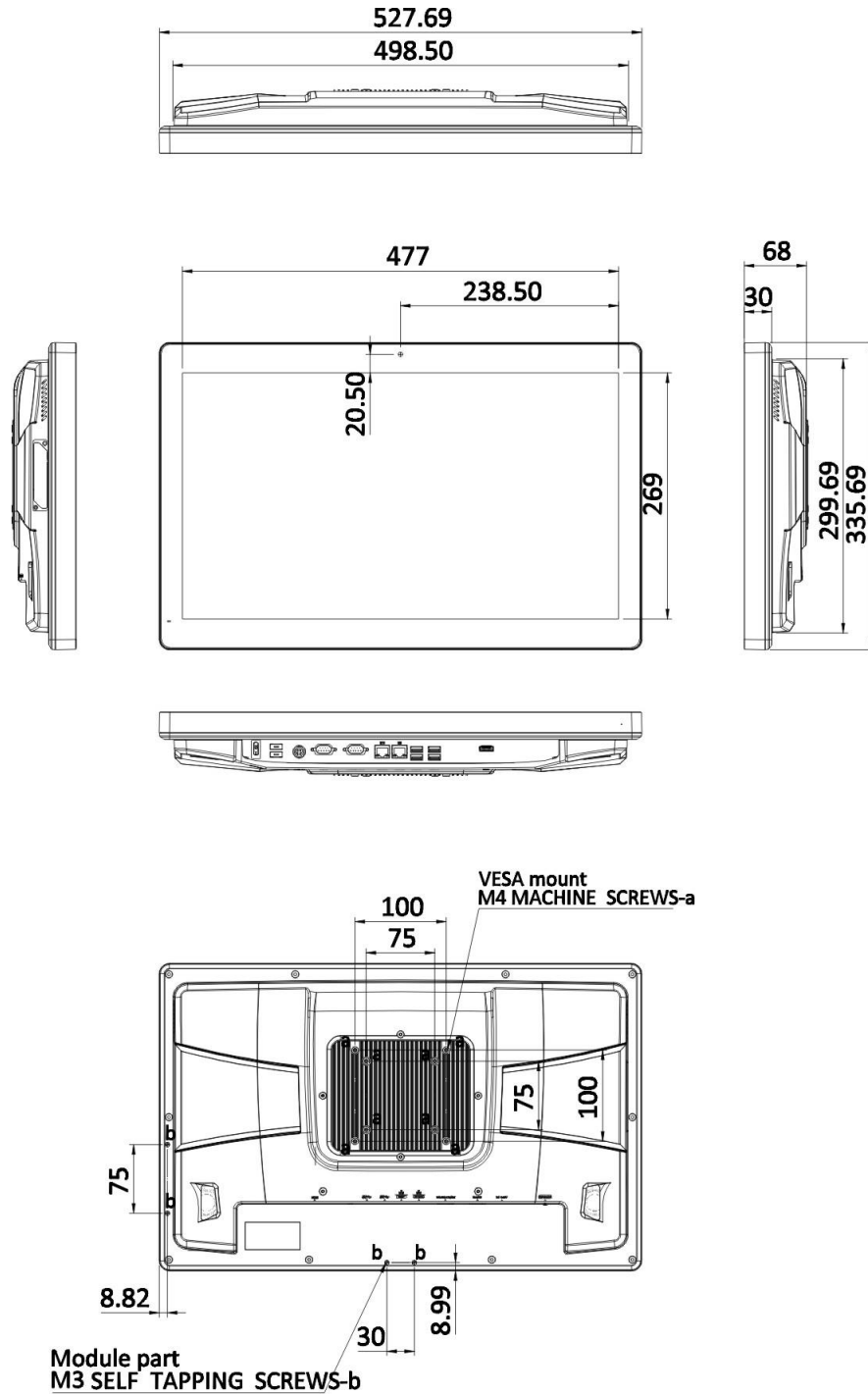
Figure 1-7: AFL3-W22C-ULT5 Dimensions (mm)
