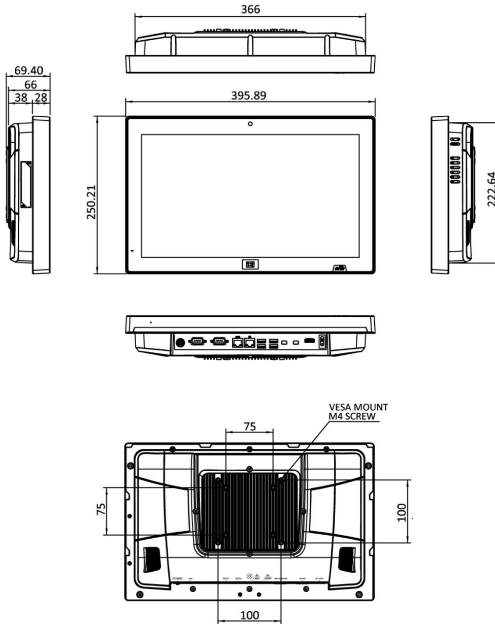
Figure 1-5: AFL3-W15C-ULT5 Dimensions (mm)
