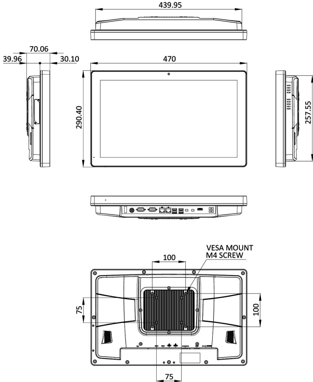
Figure 1-6: AFL3-W19C-ULT5 Dimensions (mm)
